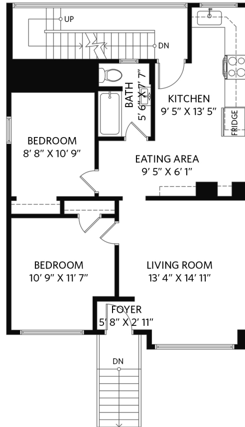
Main Floor - 895 sq.ft. Ceiling height - 7' 11" to 8' 5"
